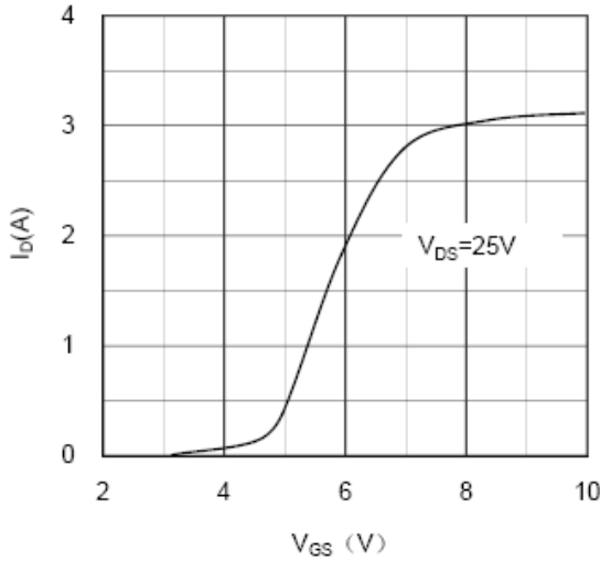
Figure 1. Transfer characteristics
